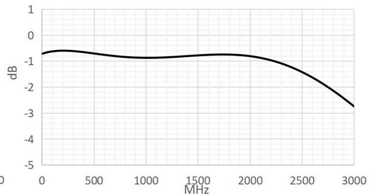
Insertion Loss:Pin 4 to 3
