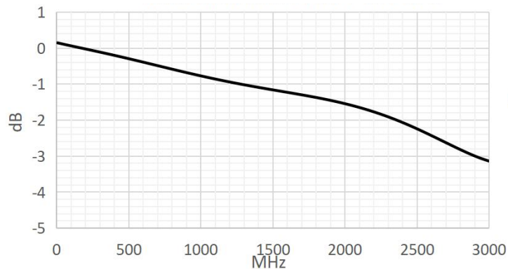
Insertion Loss:Pin 4 to 3
