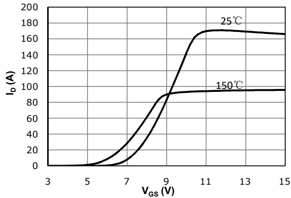
Fig 3: Transfer Characteristics
