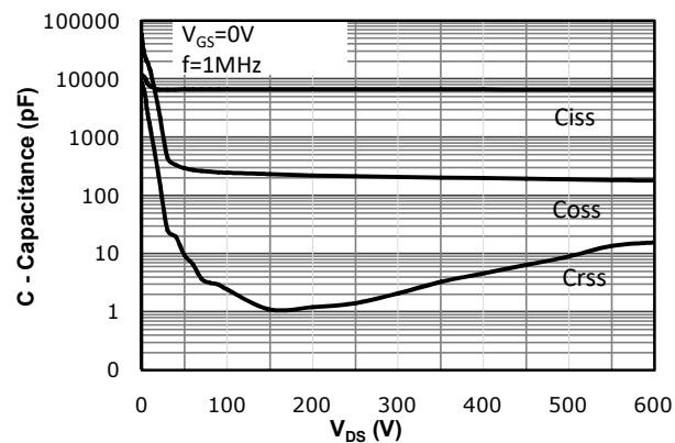
Fig 11: Capacitance Characteristics
