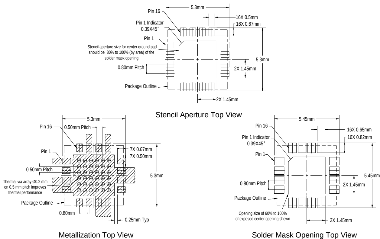
Figure 6.PCB Layout Footprint
